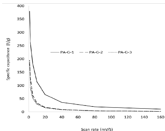
Fig. 2. Specific capacitance of composites against the scan rate
