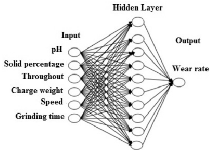
Fig. 2. BPNN architecture (6-10-1)
