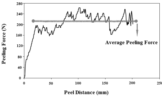
Fig. 3. Typical plot of the peeling force versus the peel distance.
