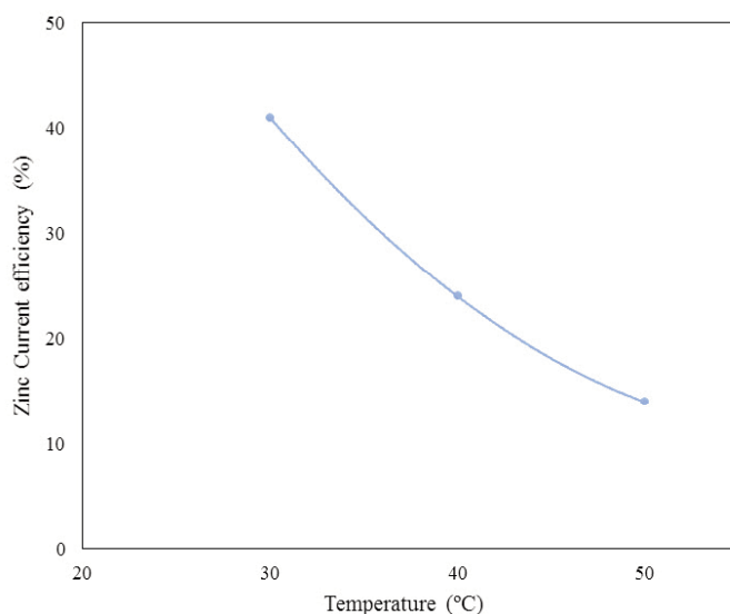
Fig. 5. Effect of plating bath temperature on partial current efficiency of Zn deposition.
