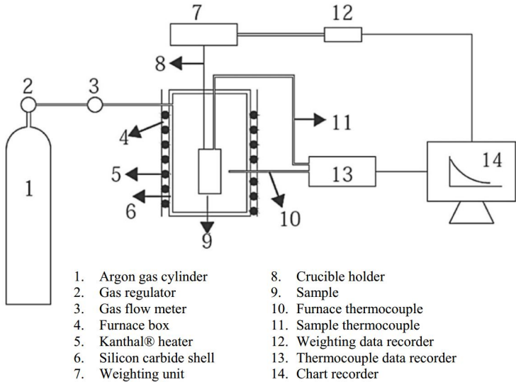
Fig. 1. Schematic thermal gravimeter furnace (TGF).
