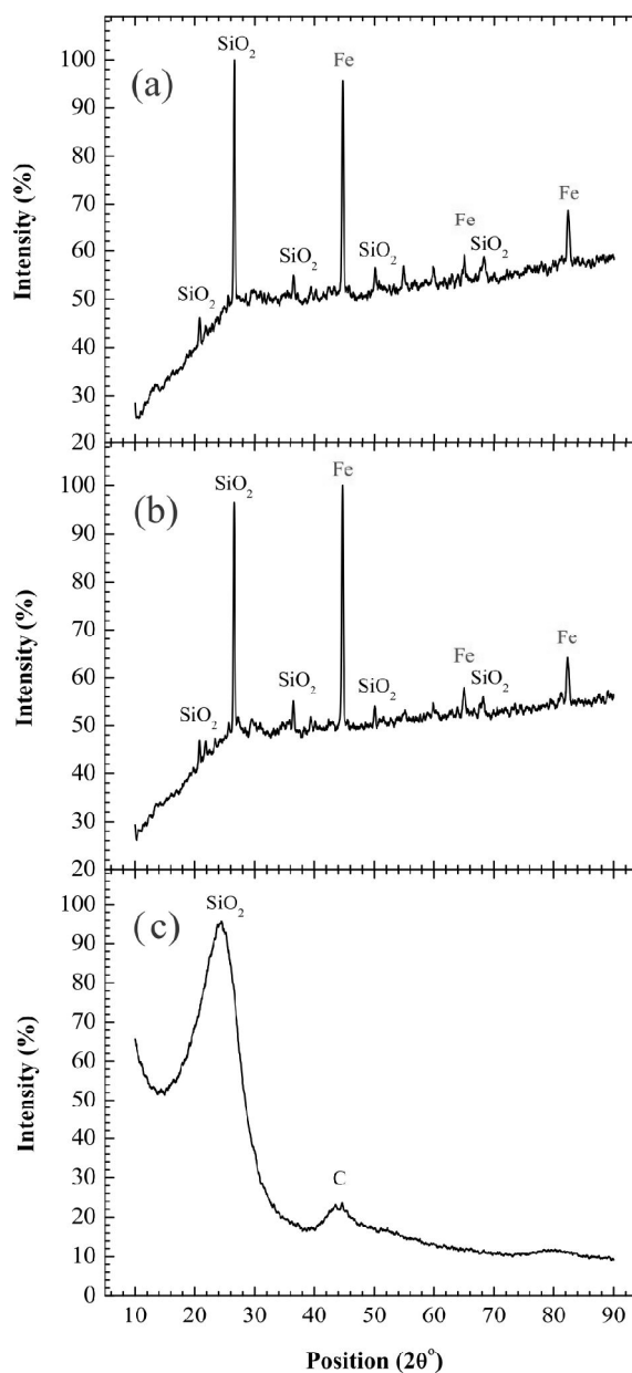
Fig. 5. XRD patterns of the sample with maximum reduction degree (96%), reduced under optimal conditions (1050°C, 3hours, 125% of stoichiometry value of required coal for complete hematite reduction). (a) Before magnetic separation, (b) Magnetic part and (c) Non-magnetic part after separation.
