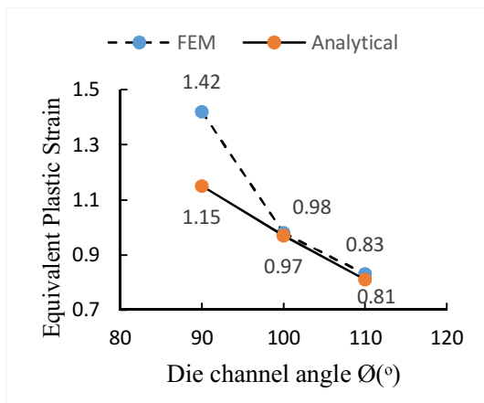
Fig. 5. Comparing the analytical and FE results for equivalent plastic strain (PEEQ) and different channel angle of 90°, 100°, 110°.
