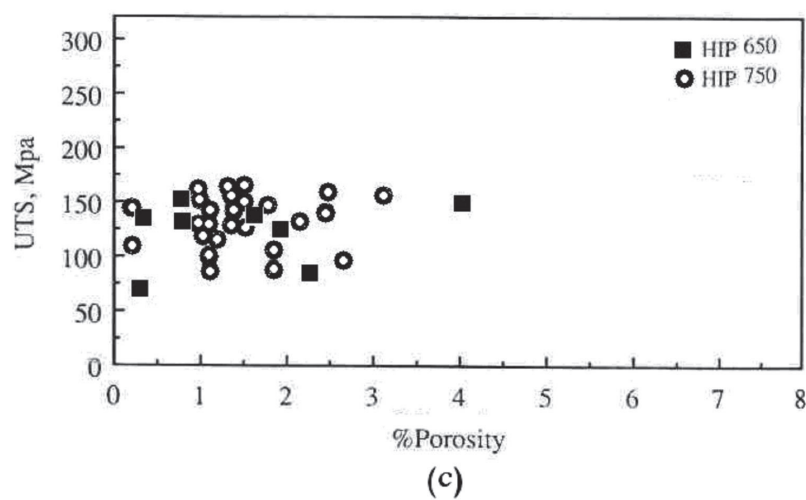
Fig. 4. The variations of UTS values as a function of porosity in A356 specimens. a) as-cast; b) age hardened; c) hipped specimens.
