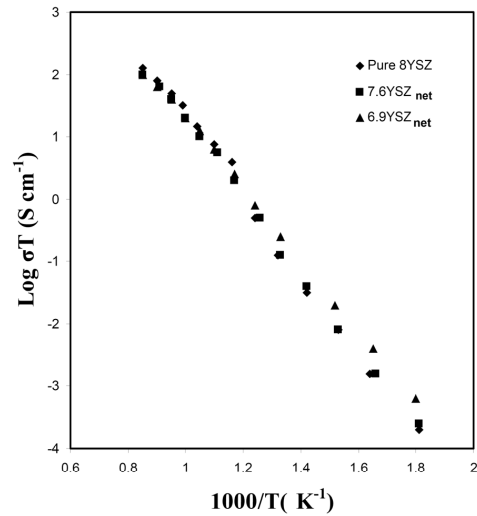
Fig. 6. Temperature dependence of bulk conductivity of samples at low temperatures ( T < 550^\circ\text{C} )
