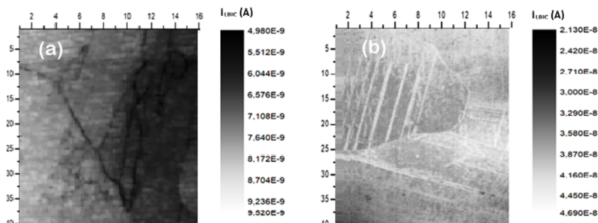
Fig. 6. a) Two-dimensional Generated Current I_{\text{LBIC}} distribution before AVE max value 9.5 \times 10^{-9} A b) after AVE max value 46.9 \times 10^{-9} A.
