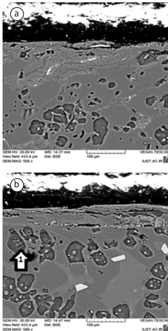
Fig.13. The subsurface area of the Specimens worn at the applied loads of (a) 25N and (b) 75N. Cracks in particle shown by arrow numbered 1. Formation of tribolayer (MML) during the wear process can be apparently seen.
